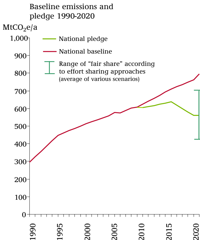
Fig. 6: South Korea: Projected BAU and pledged emissions compared to results from effort sharing approaches
