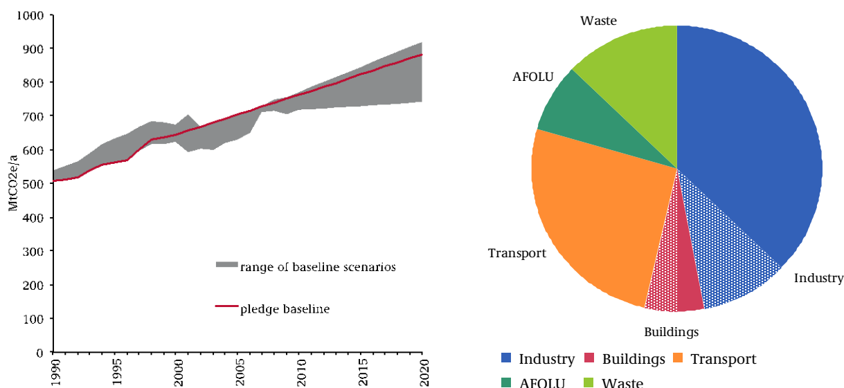
Fig. 26: Mexico: Historical GHG emissions and projections from 1990 until 2020 (CO 2 , CH 4 , N 2 O, HFCs, PFCs, SF 6 ). Pie chart on the right shows distribution of emissions to sectors expected in 2020. Shaded areas are electricity related emissions.
