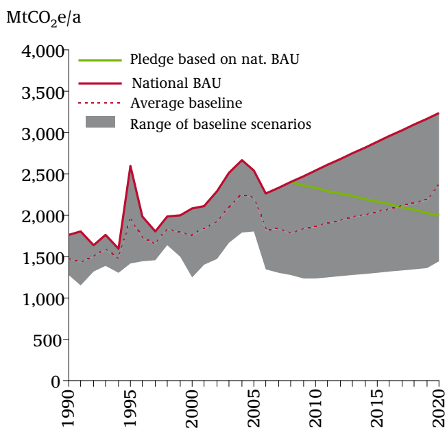
Fig. 13: Estimated emissions resulting from Brazil's pledge
