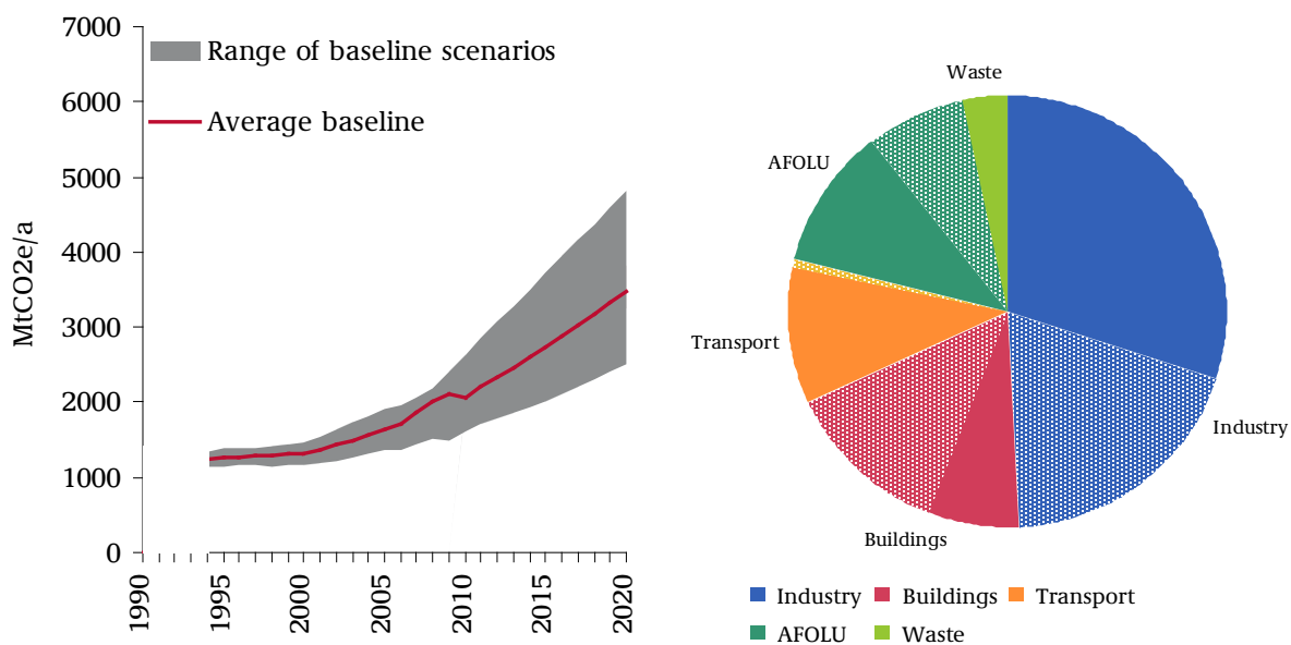
Fig. 21: India: Historical GHG emissions and projections from 1990 until 2020 (CO 2 , CH 4 , N 2 O, HFCs, PFCs, SF 6 ). Pie chart on the right shows distribution of emissions to sectors as in 2020. Shaded areas are electricity related emissions
